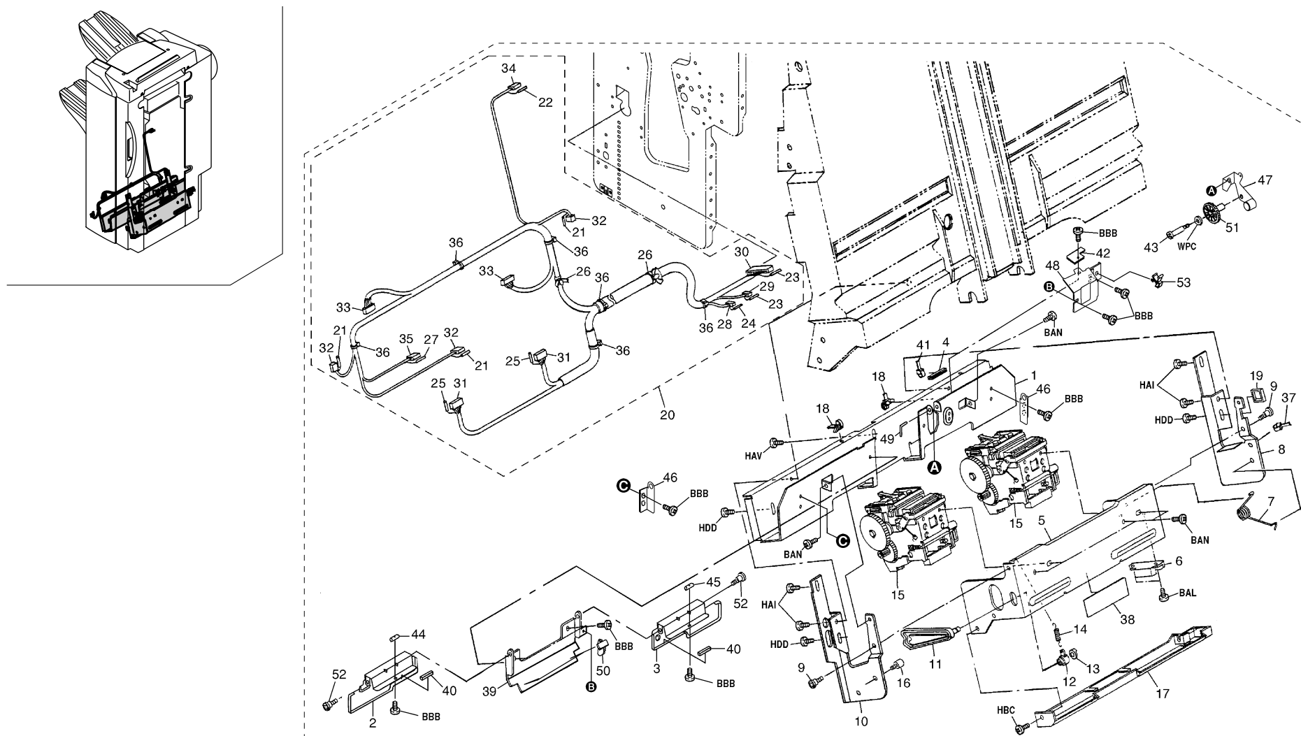
FIG. 7 MIDDLE TRAY II
